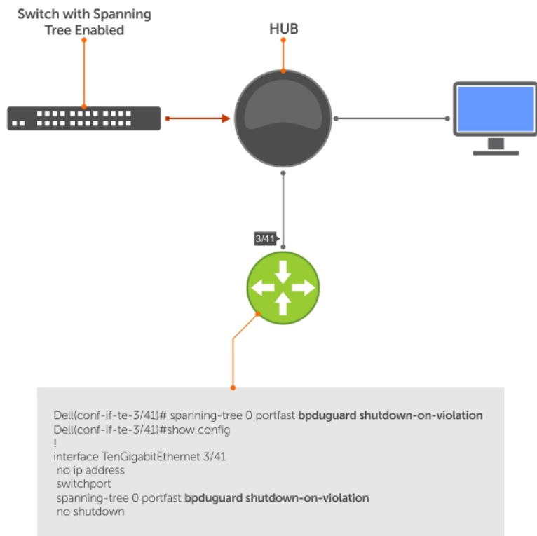
Figure 117. Enabling BPDUGuard
