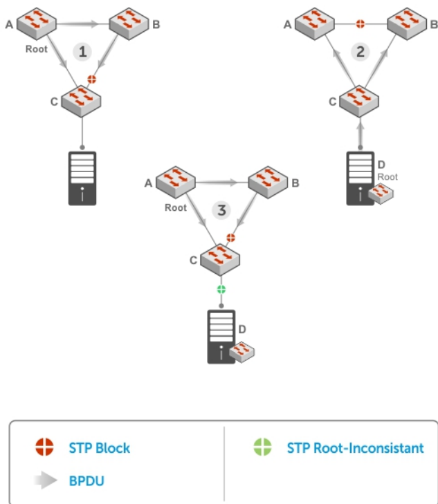
Figure 118. STP Root Guard Prevents Bridging Loops
