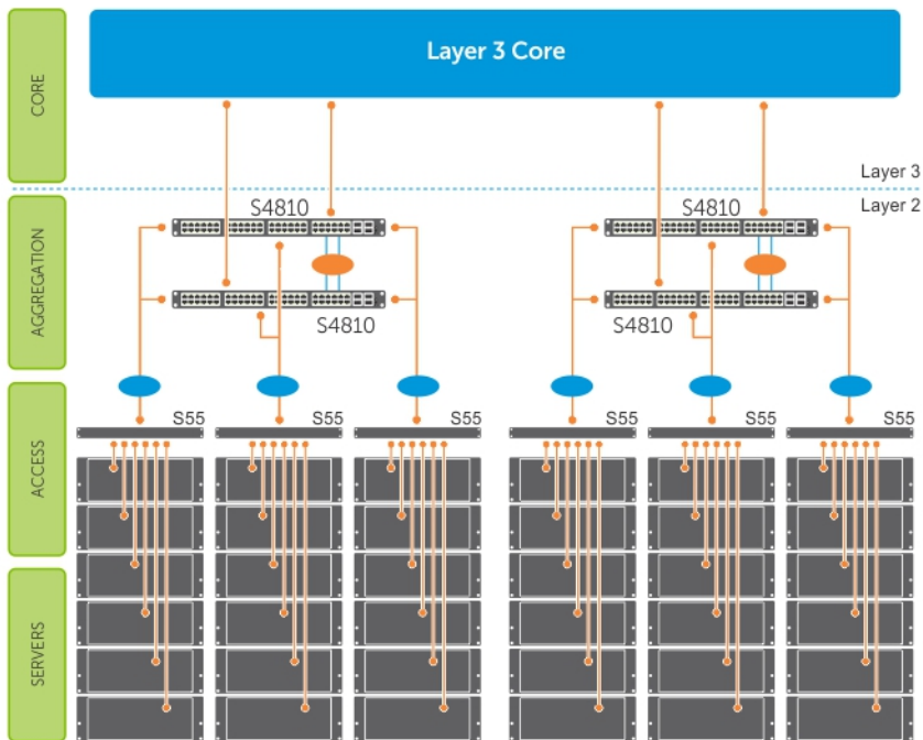
Figure 123. Enhanced VLT
