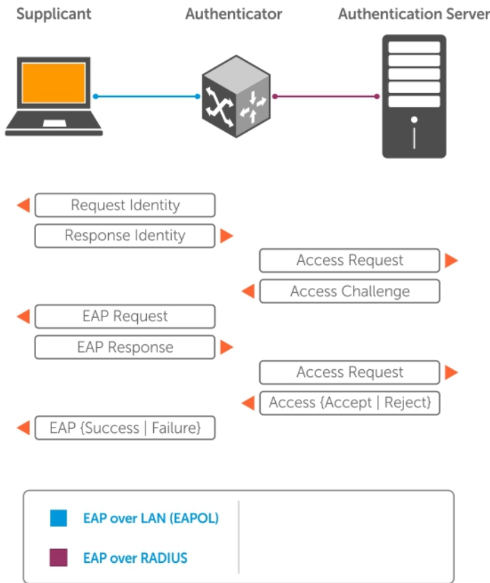
Figure 4. EAP Port-Authentication
