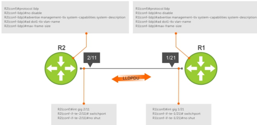
Figure 73. Configuring LLDP
