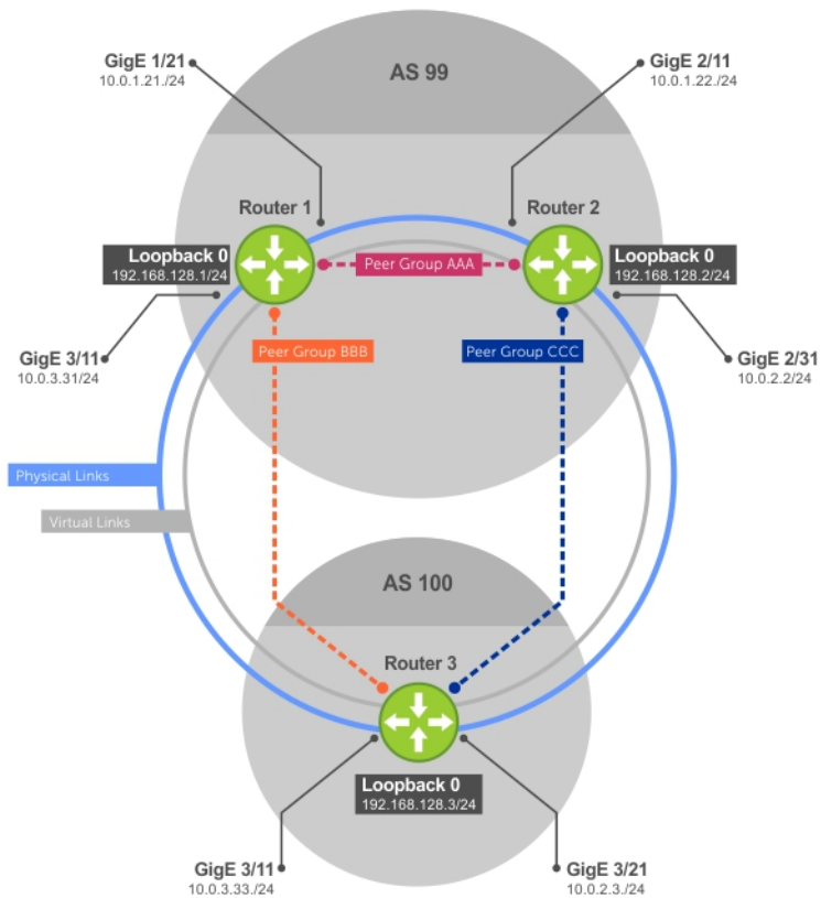
Figure 24. Sample Configurations
