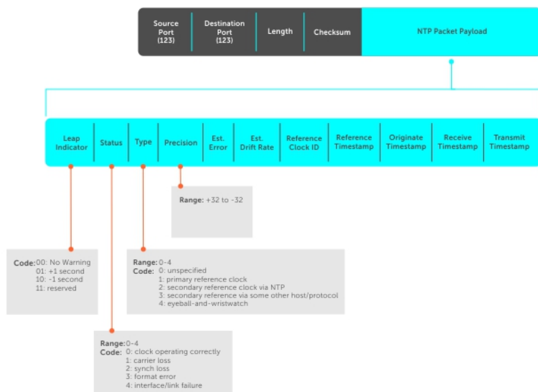
Figure 120. NTP Fields
