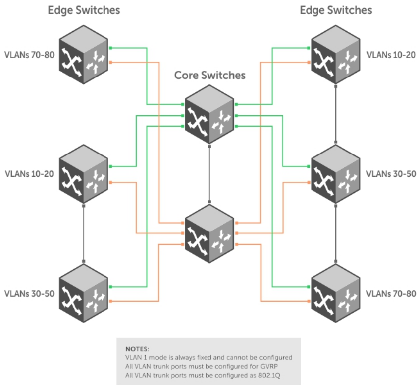
Figure 37. Global GVRP Configuration Example
