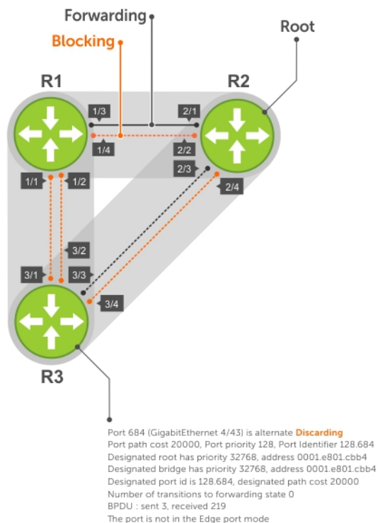
Figure 104. Rapid Spanning Tree Enabled Globally
