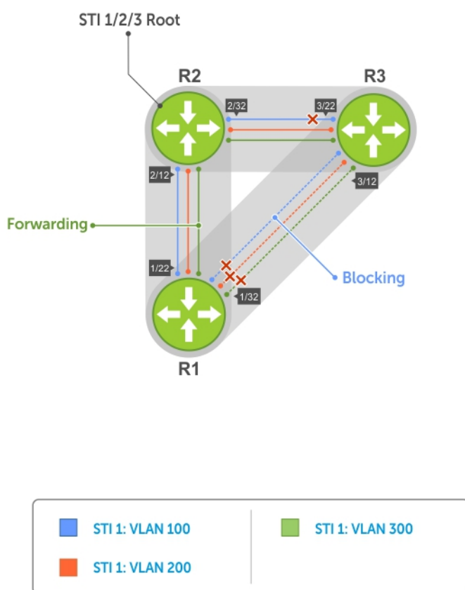
Figure 97. Per-VLAN Spanning Tree
