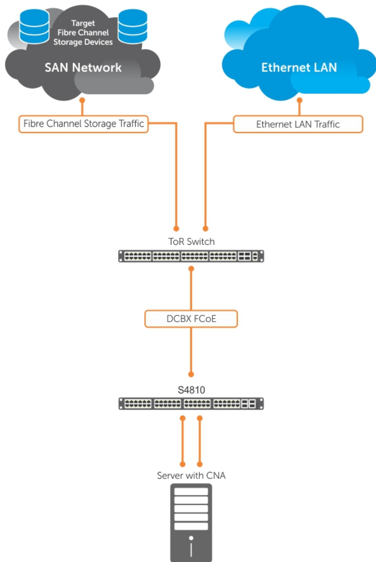
Figure 35. FIP Snooping on an S6000 Switch
