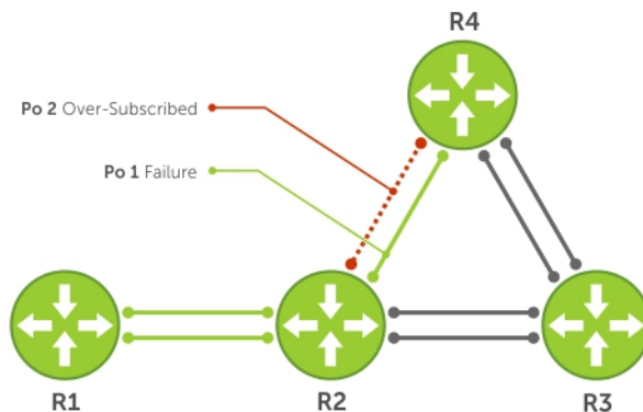
Figure 54. Shared LAG State Tracking
