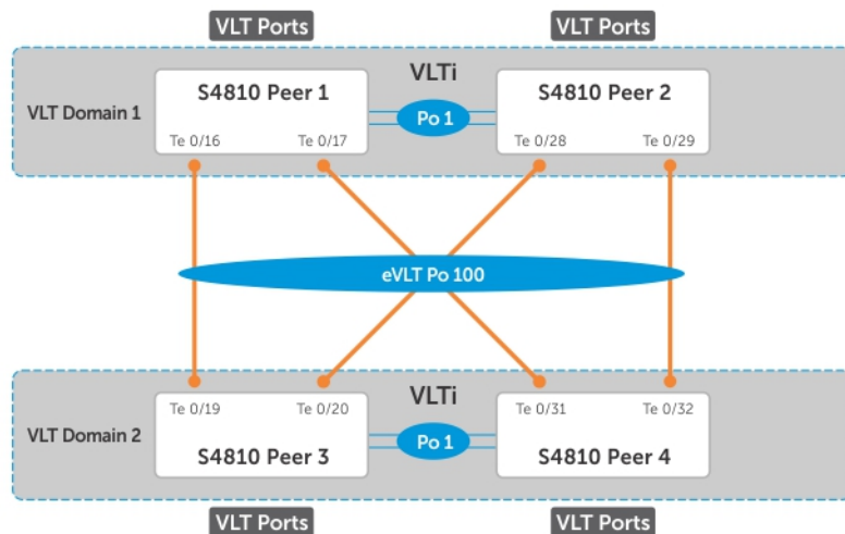
Figure 125. eVLT Configuration Example
