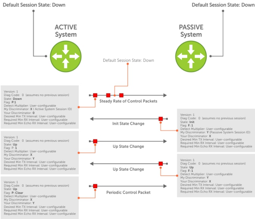
Figure 9. BFD Three-Way Handshake State Changes
