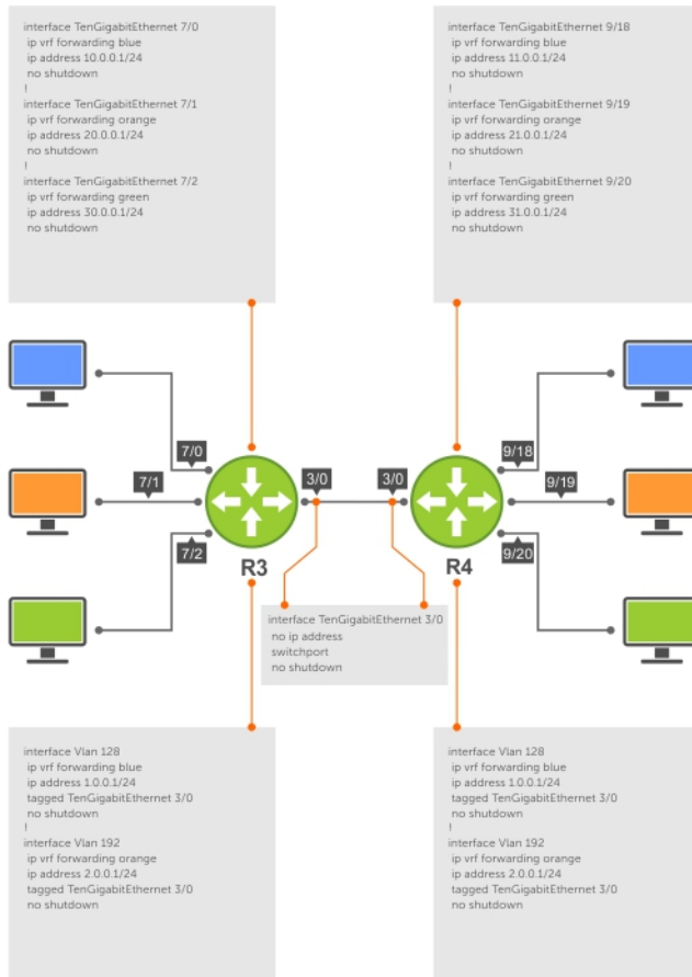
Figure 128. Setup VRF Interfaces
