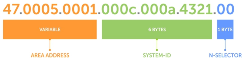
Figure 52. ISO Address Format
