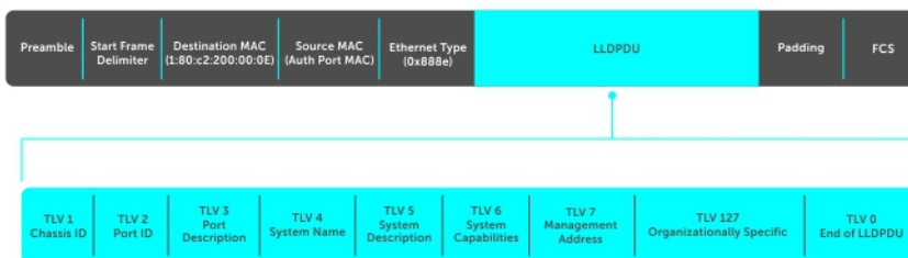
Figure 68. LLDPDU Frame
