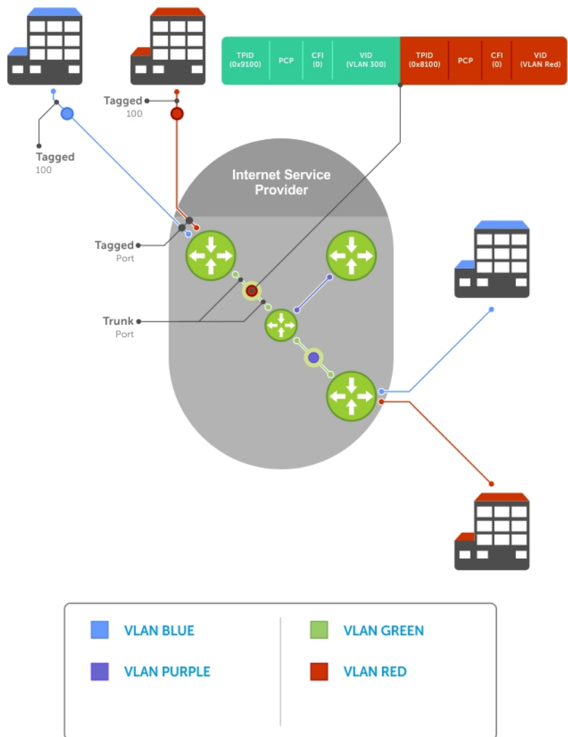
Figure 105. VLAN Stacking in a Service Provider Network
