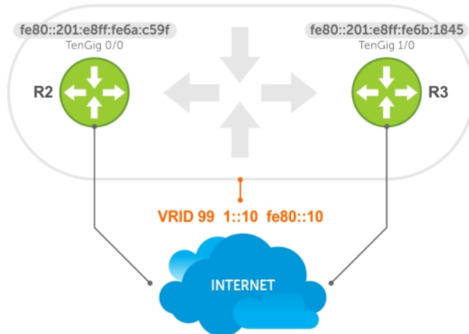
Figure 131. VRRP for an IPv6 Configuration
