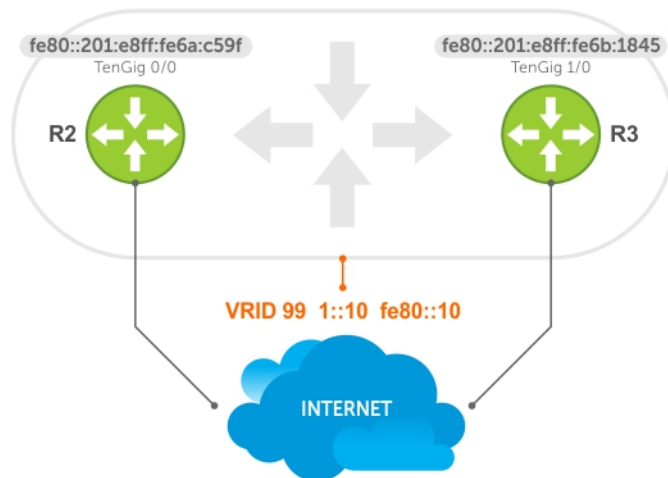
Figure 133. VRRP for IPv6 Topology
