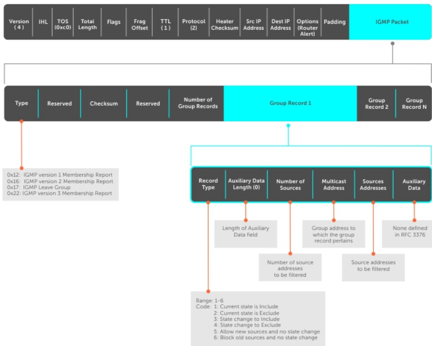
Figure 40. IGMP Version 3-Capable Multicast Routers Address Structure
