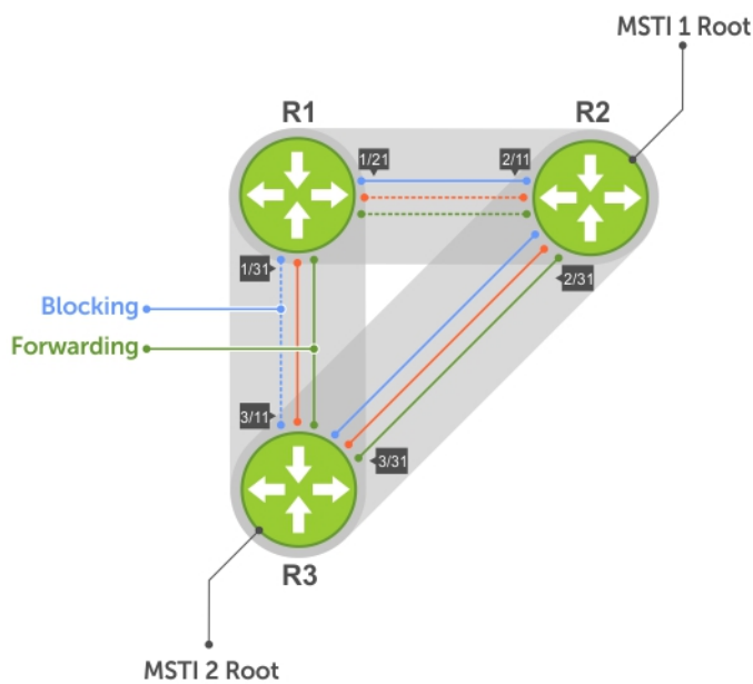
Figure 86. MSTP with Three VLANs Mapped to TWO Spanning Tree Instances
