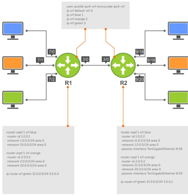
Figure 127. Setup OSPF and Static Routes
