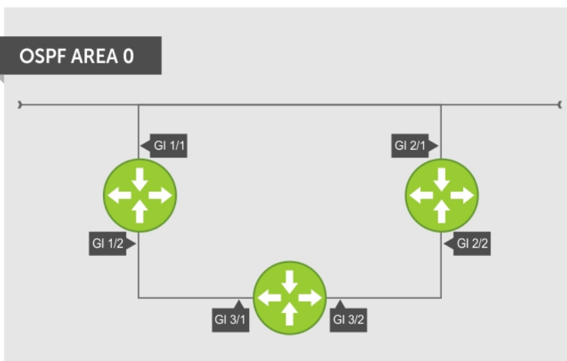
Figure 94. Basic Topology and CLI Commands for OSPFv2
