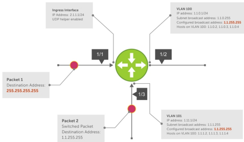
Figure 47. UDP Helper with Configured Broadcast Addresses
