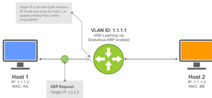
Figure 44. ARP Learning via ARP Request with ARP Learning via Gratuitous ARP Enabled
