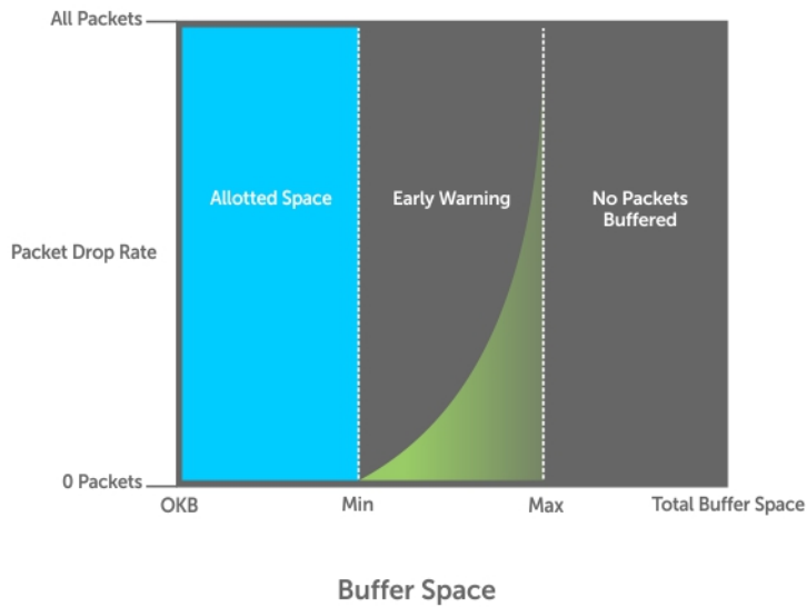
Figure 102. Packet Drop Rate for WRED
