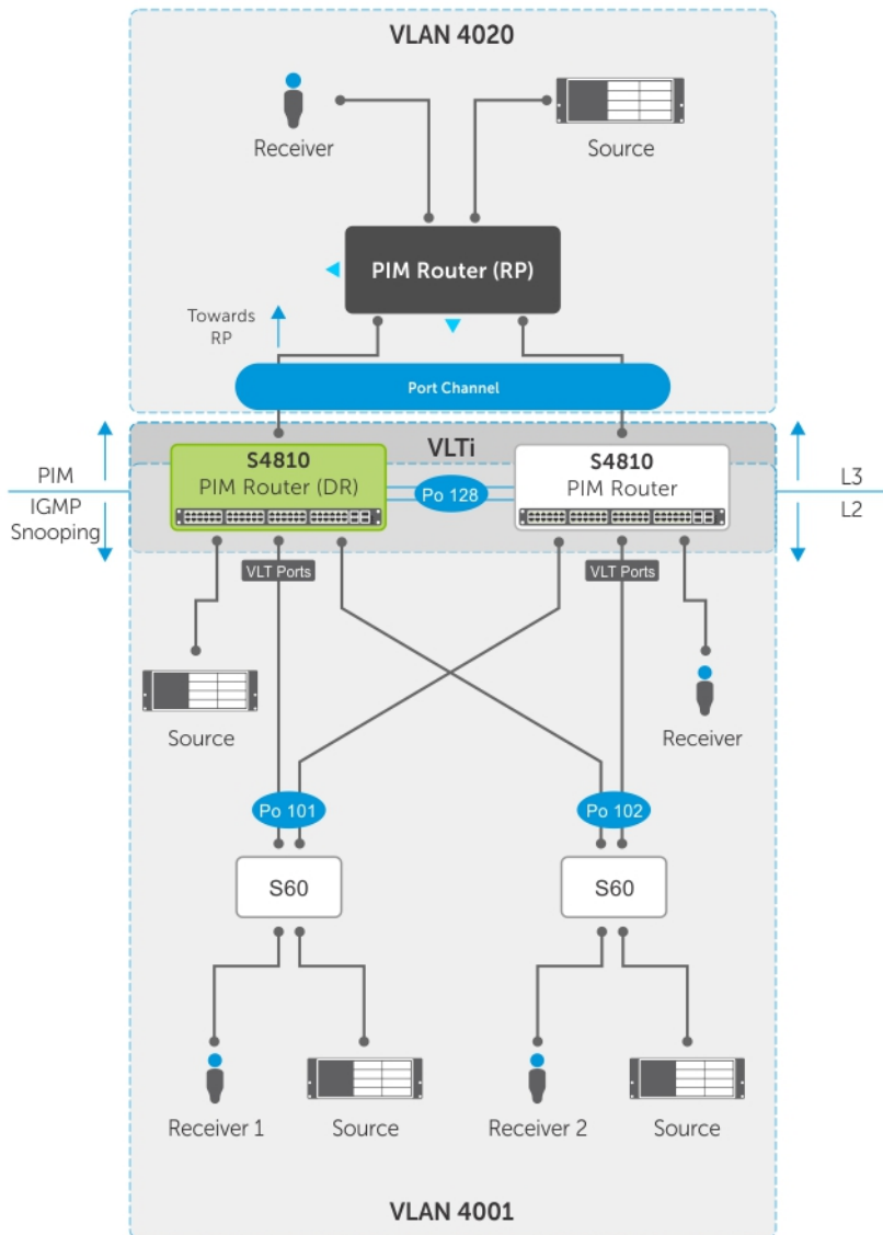
Figure 124. PIM-Sparse Mode Support on VLT
