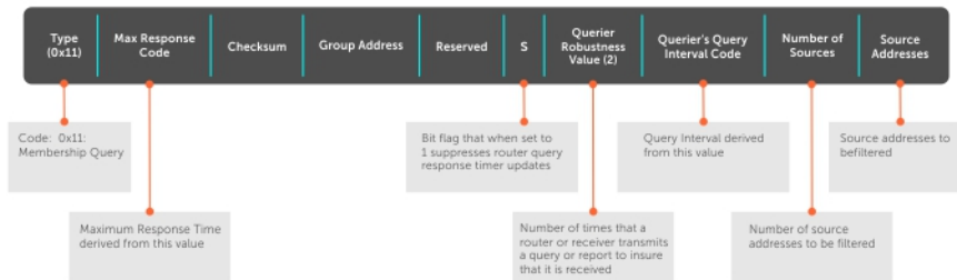
Figure 39. IGMP Version 3 Packet Structure
