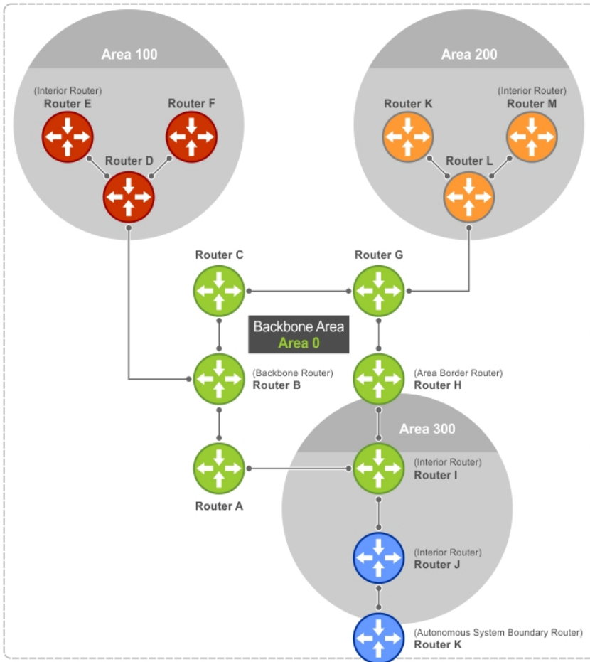
Figure 91. Autonomous System Areas
