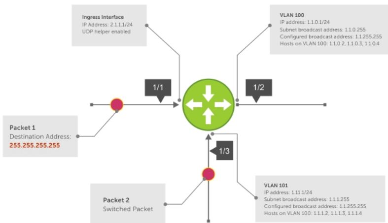
Figure 45. UDP Helper with Broadcast-All Addresses
