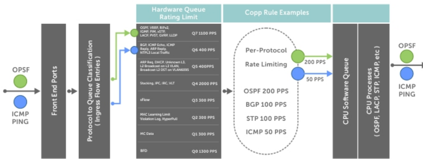
Figure 25. Control Plane Policing
