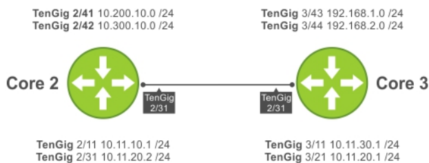
Figure 103. RIP Topology Example
