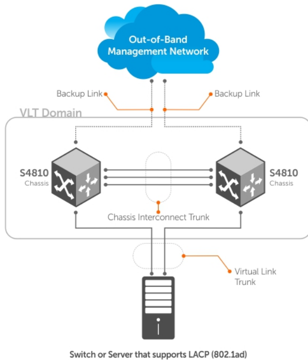
Figure 122. VLT on Switches
