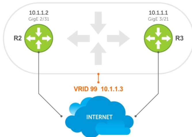
Figure 130. VRRP for IPv4 Topology
