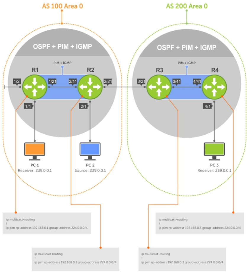
Figure 79. Configuring PIM in Multiple Routing Domains
