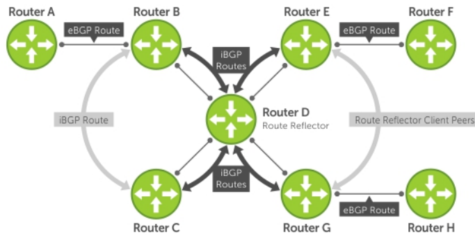
Figure 19. BGP Router Rules
