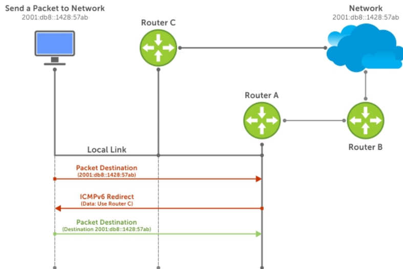
Figure 50. NDP Router Redirect
