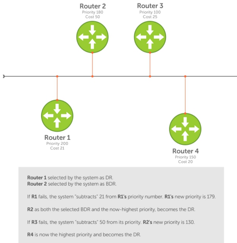
Figure 93. Priority and Cost Examples
