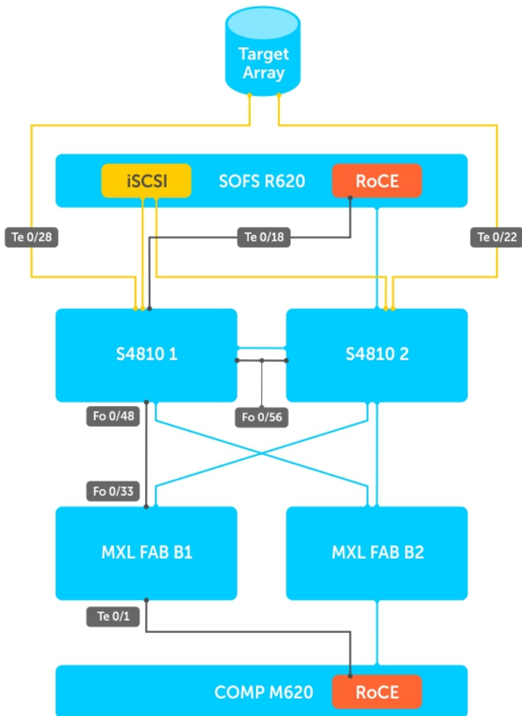
Figure 31. Configure DCB end to end on this setup
