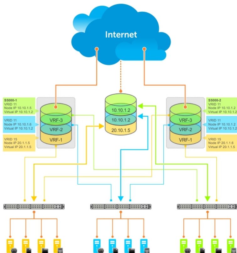
Figure 132. VRRP in a VRF: Non-VLAN Example
