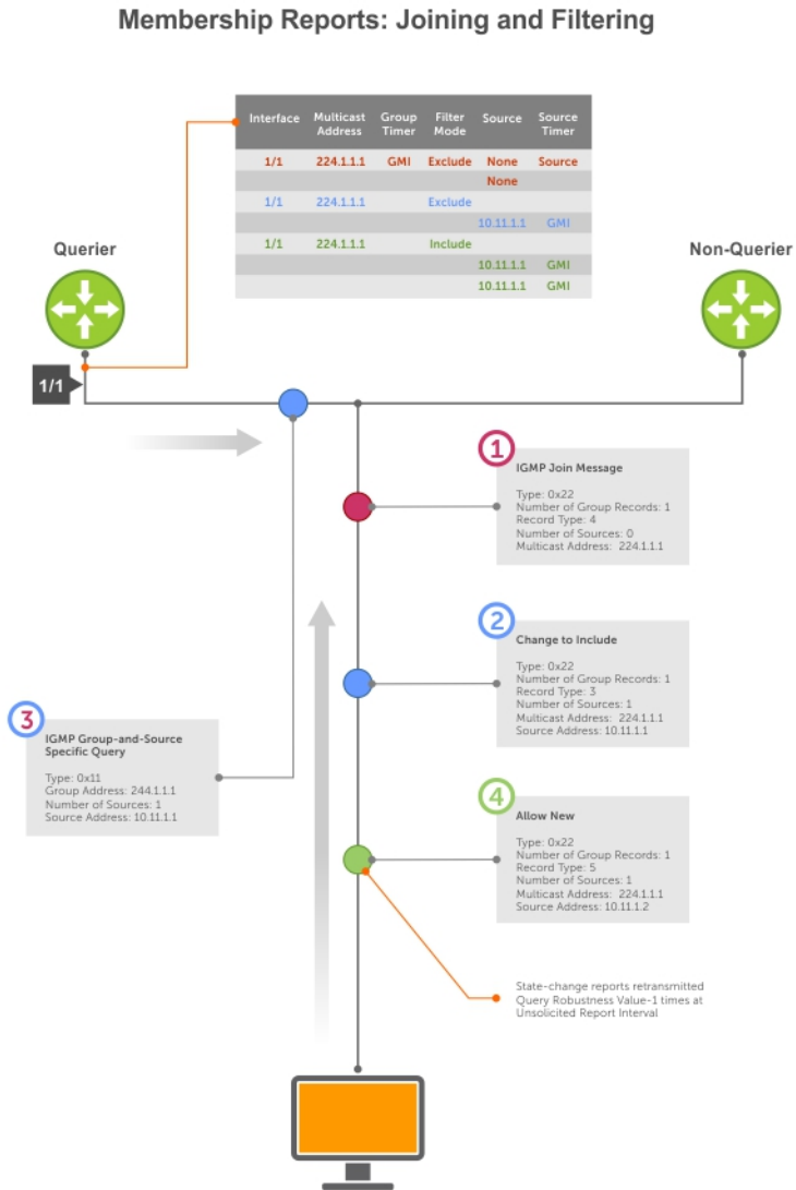
Figure 41. Membership Reports: Joining and Filtering
