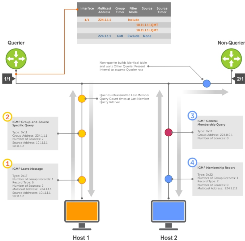
Figure 42. Membership Queries: Leaving and Staying
