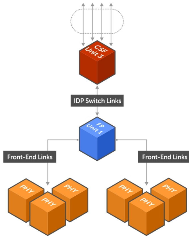
Figure 135. Buffer Tuning Points
