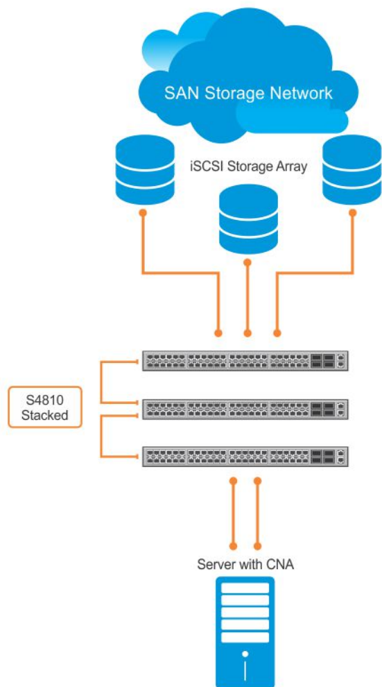
Figure 51. iSCSI Optimization Example
