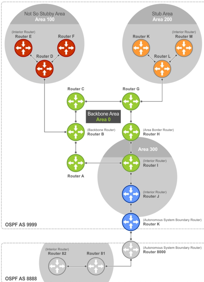
Figure 92. OSPF Routing Examples
