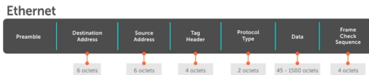
Figure 121. Tagged Frame Format
