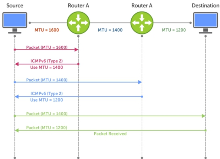
Figure 49. Path MTU Discovery Process
