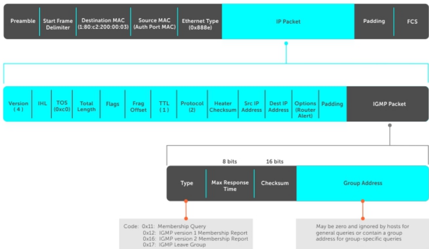
Figure 38. IGMP Messages in IP Packets
