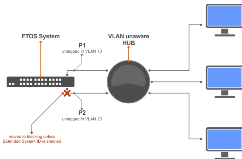
Figure 99. PVST+ with Extend System ID
