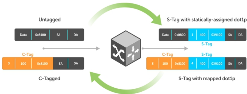
Figure 109. Statically and Dynamically Assigned dot1p for VLAN Stacking
