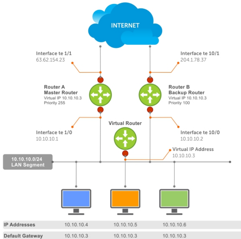
Figure 129. Basic VRRP Configuration
