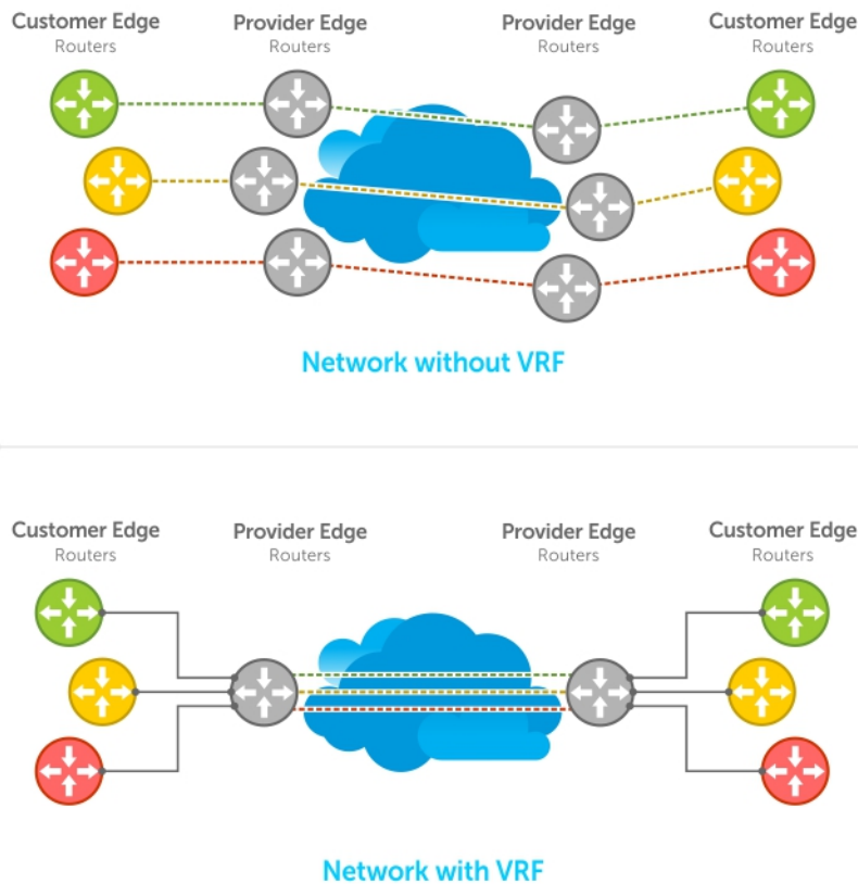
Figure 126. VRF Network Example
