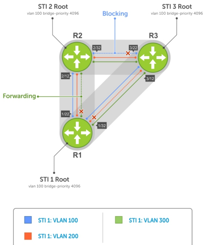
Figure 98. Load Balancing with PVST+
