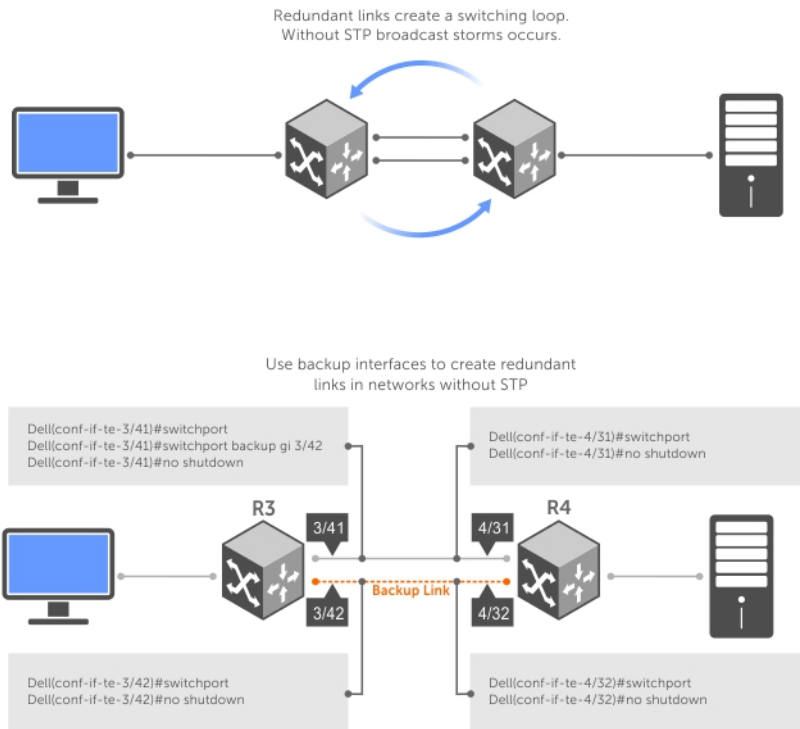
Figure 65. Configuring Redundant Layer 2 Pairs without Spanning Tree
