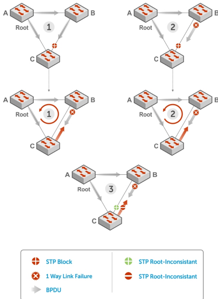
Figure 119. STP Loop Guard Prevents Forwarding Loops
