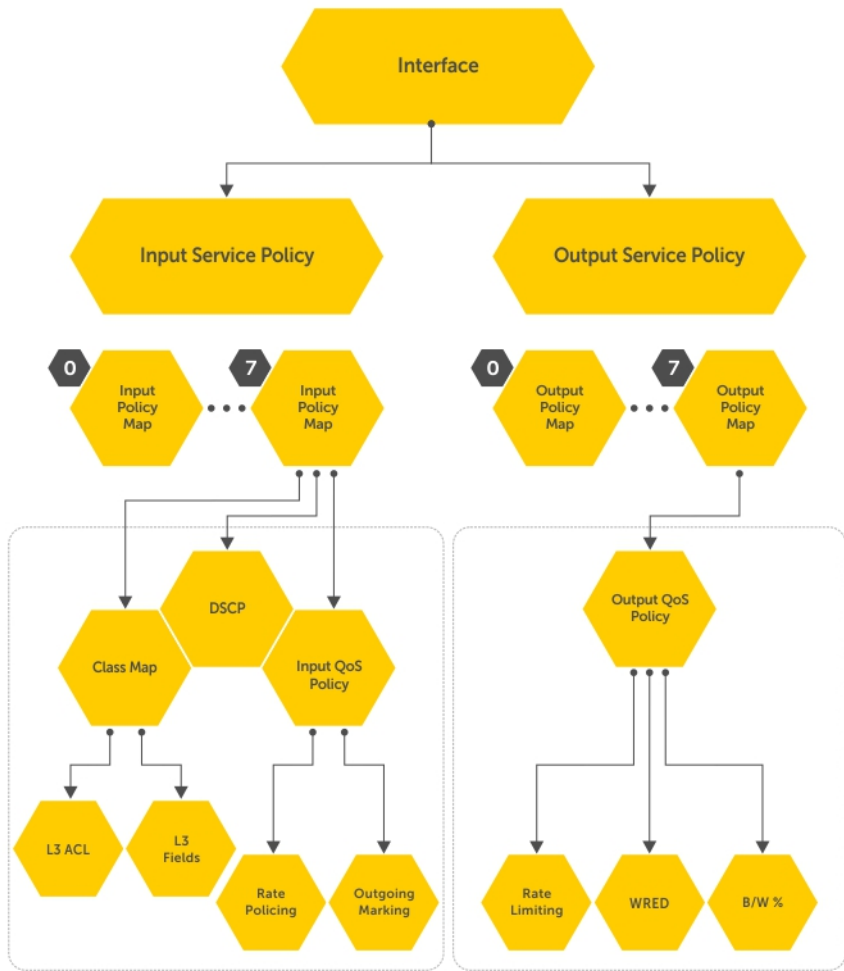
Figure 101. Constructing Policy-Based QoS Configurations
