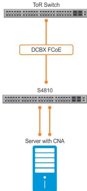
Figure 36. Configuration Example: FIP Snooping on a Switch
