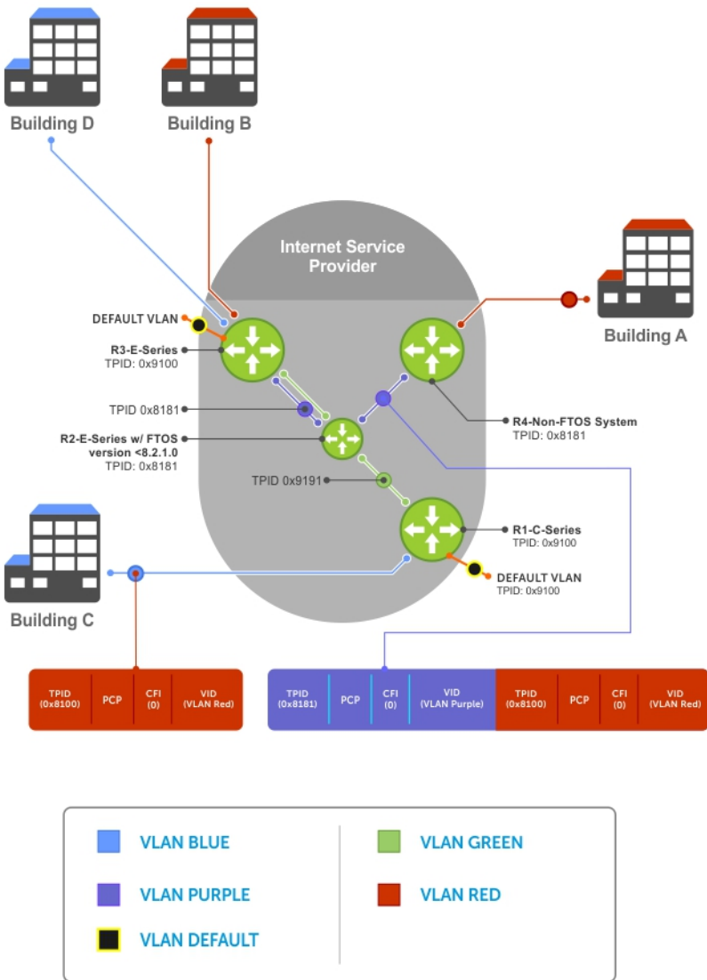
Figure 108. Single and Double-Tag TPID Mismatch
