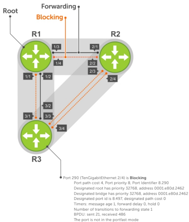
Figure 116. Spanning Tree Enabled Globally
