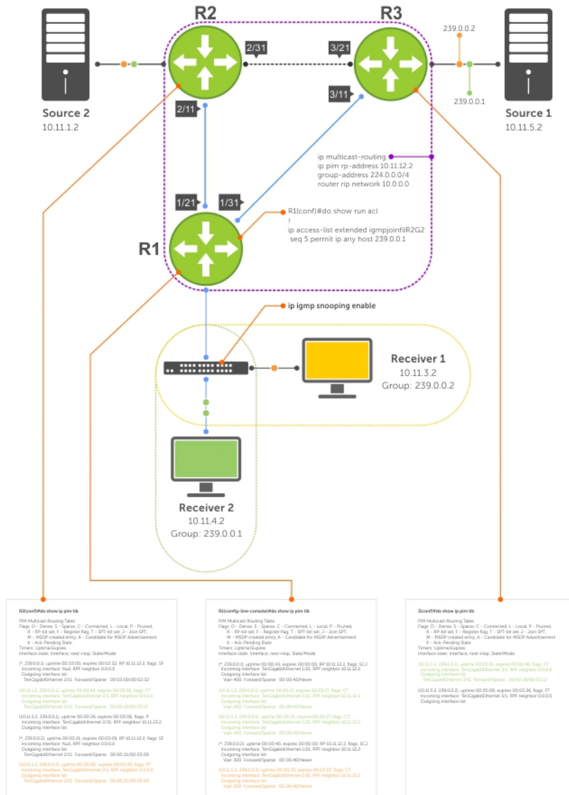
Figure 89. Preventing a Source from Transmitting to a Group
