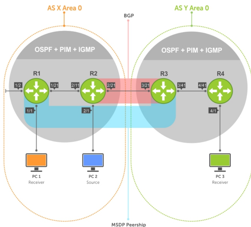
Figure 75. Multicast Source Discovery Protocol (MSDP)
