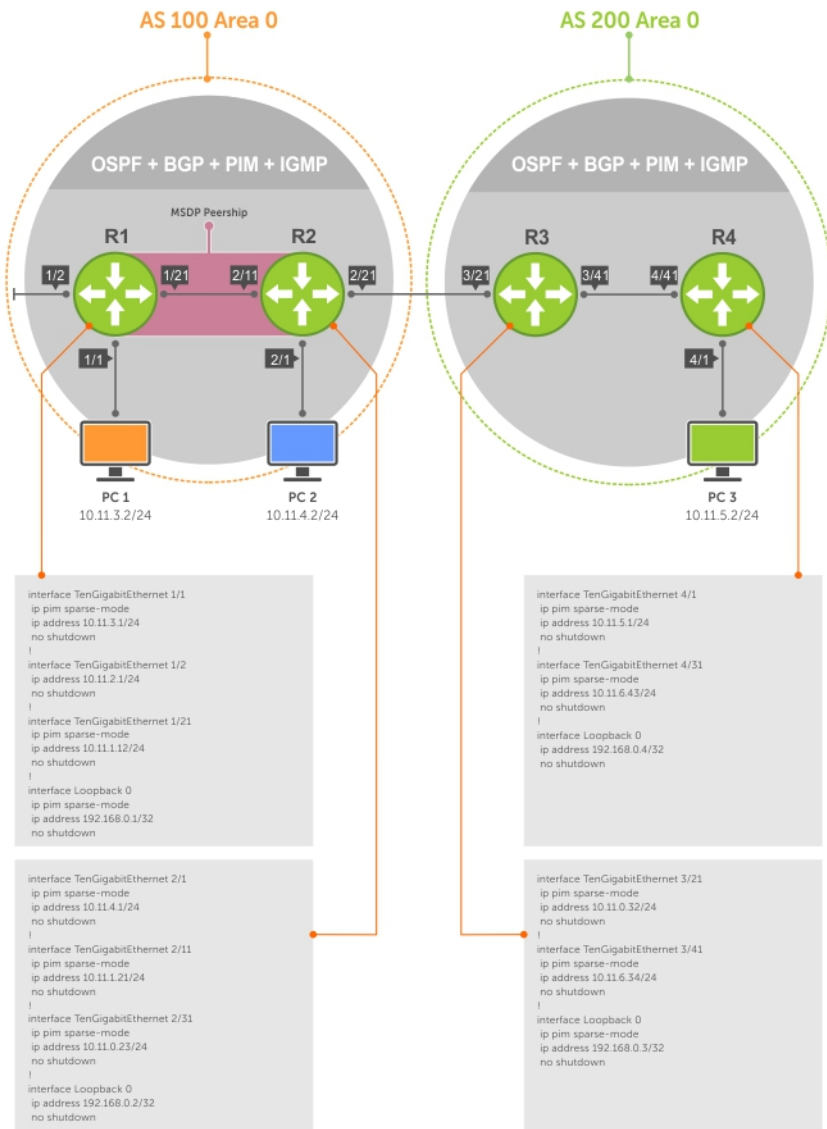
Figure 80. Configuring MSDP
