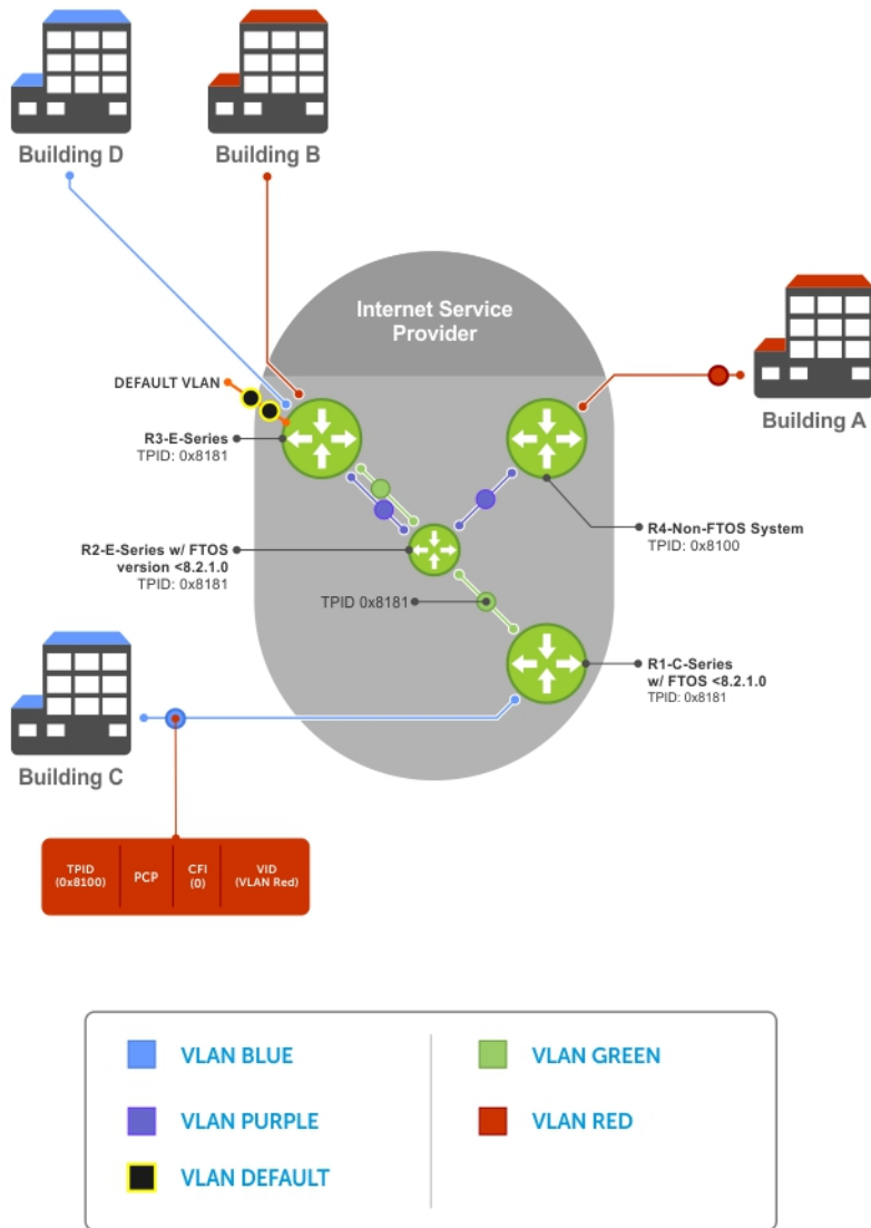
Figure 107. Single and Double-Tag First-byte TPID Match
