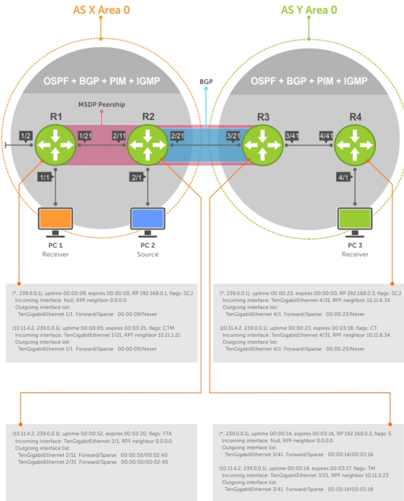
Figure 85. MSDP with Anycast RP
