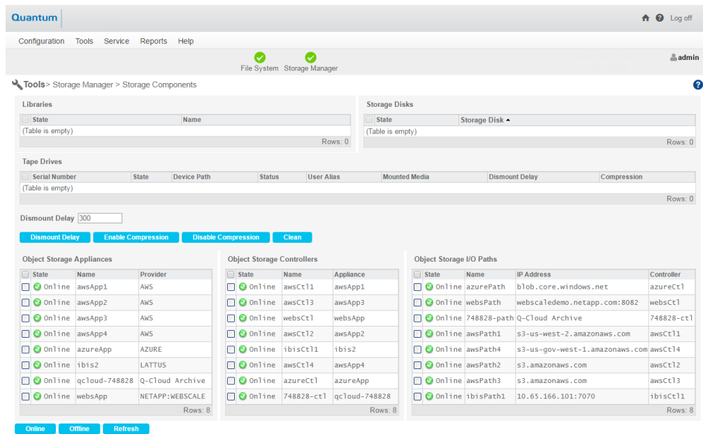
Figure 14: Tools > Storage Manager > Storage Components Page
