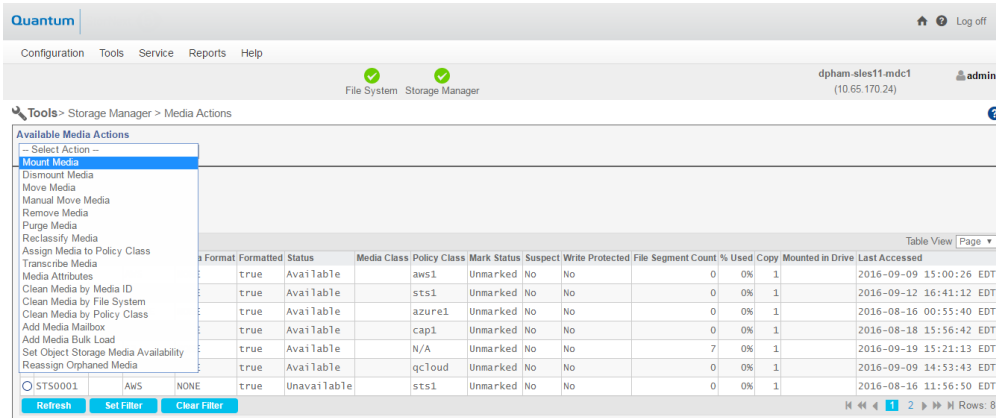
Figure 16: Tools > Storage Manager > Media Actions (Available Media Actions list) Page
