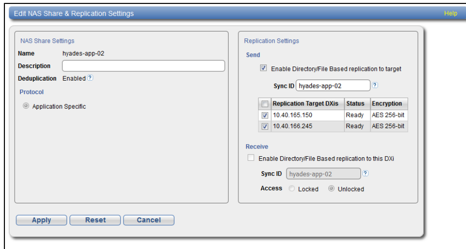
Figure 6: Edit NAS Share & Replication Settings Page
