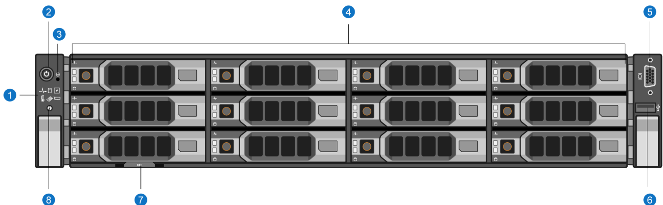
Figure 10: DXi4700 G1 Node - Front View
