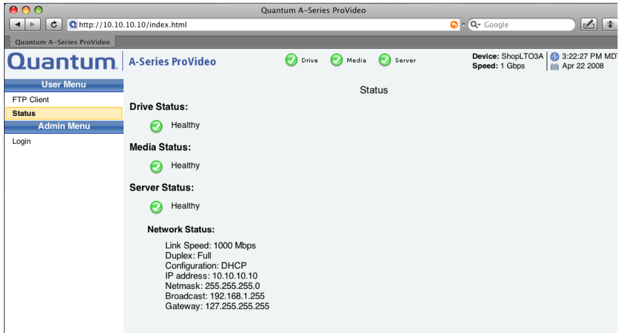
Figure 12 Status Page
