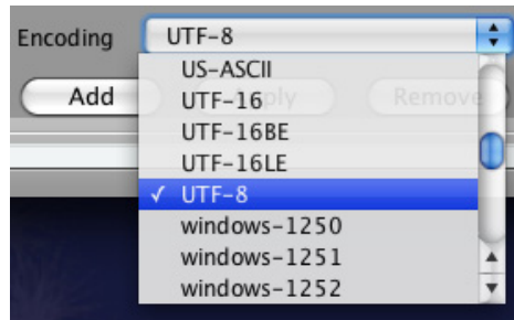
Figure 20 Encoding Schemes
