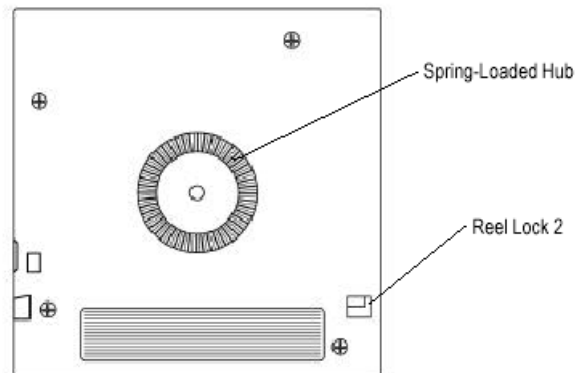
Figure B-2. Bottom View of DLT Data Cartridge
