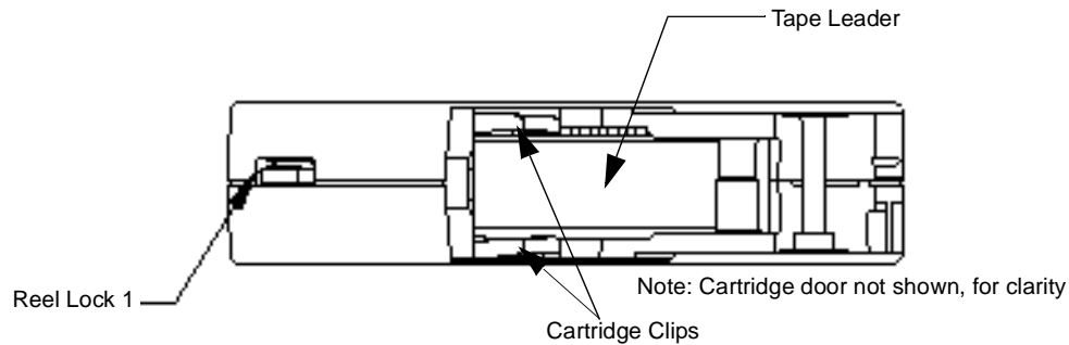
Figure A-2. End View of Super DLTtape I Data Cartridge
