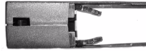
Toed-in cartridge buckling clips (extreme)
