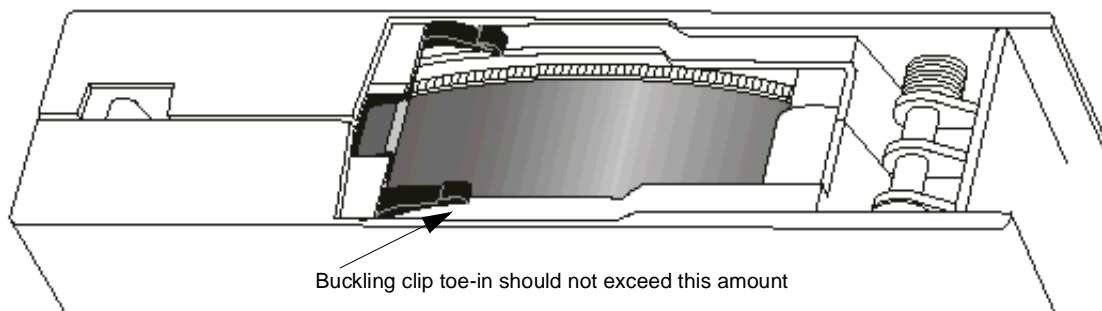
Figure A-5. CAD Diagram Showing Limit of Buckling Clip Toe-in
