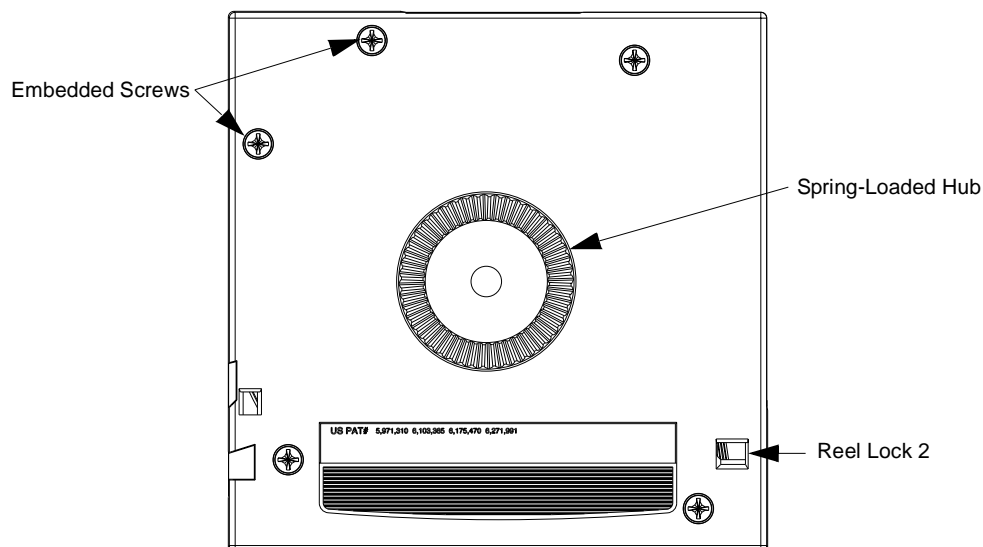
Figure A-3. Bottom View of Super DLTtape I Data Cartridge
