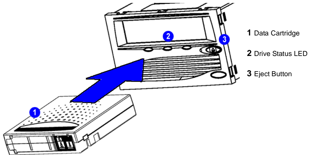
Figure A-7. Loading a Data Cartridge
