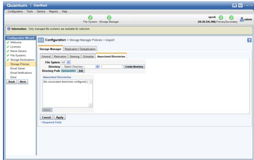
Figure 32 Storage Policies > New > Associated Directories Tab
