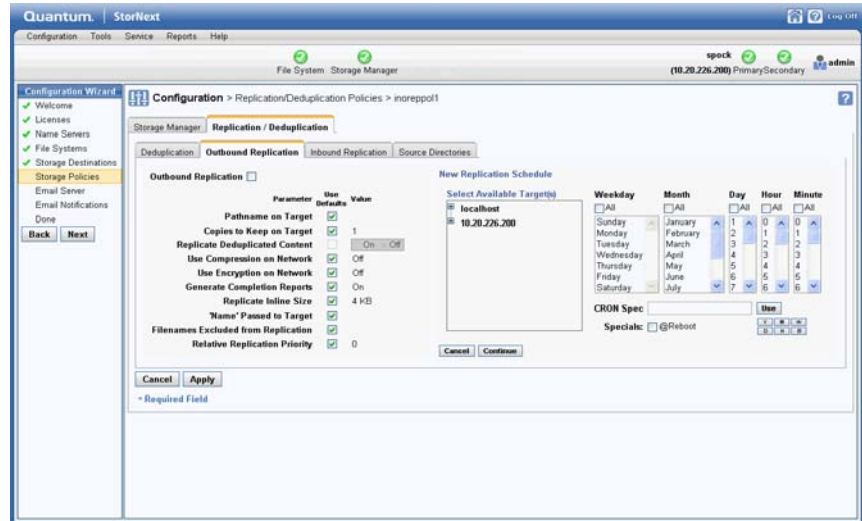
Figure 76 Outbound Replication Tab > Replication Schedule
