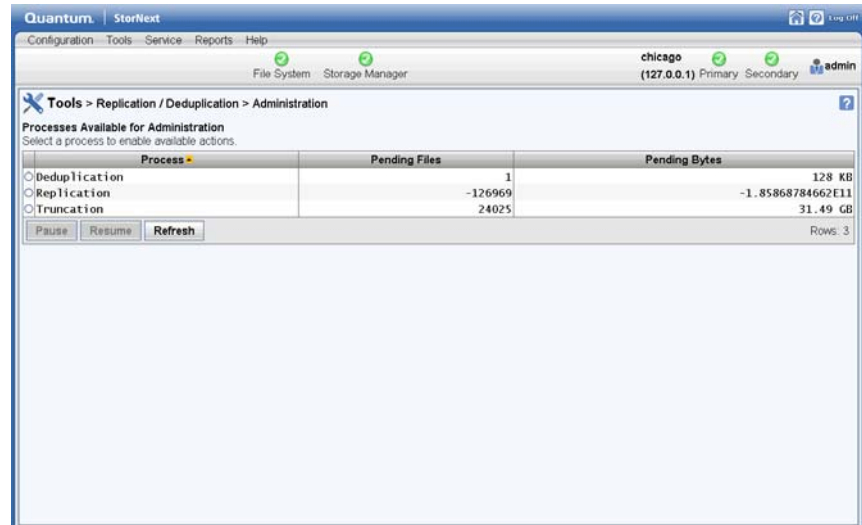
Figure 83 Tools > Replication/Deduplication > Administration Screen
