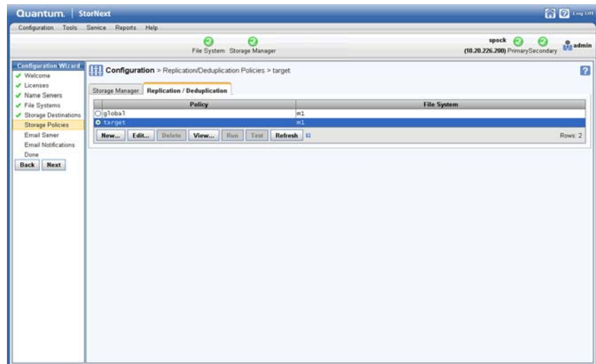
Figure 77 Configuration > Storage Policies Screen (Select "target")
