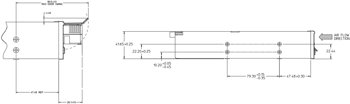
Figure 16 LTO-3 (Model B) Half-Height Drive Dimensions (side)
