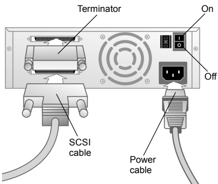
Figure 3: Back of Tape Drive
