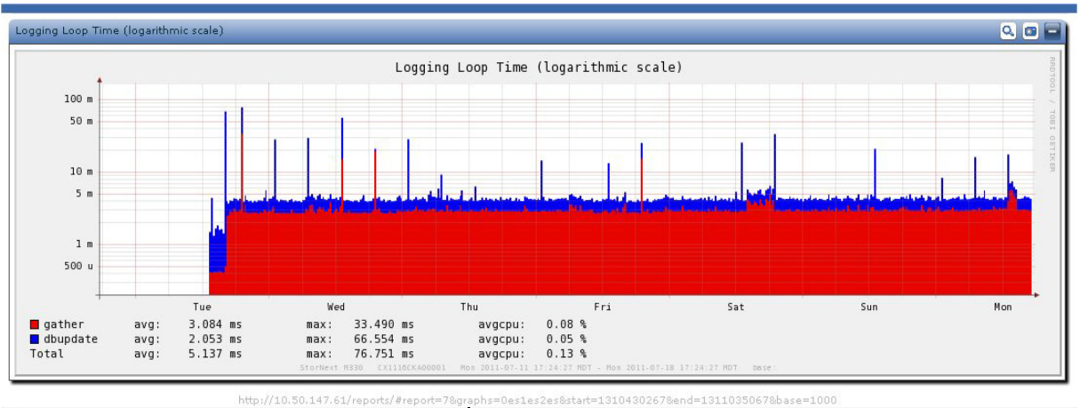
Figure 8 URL Reference
